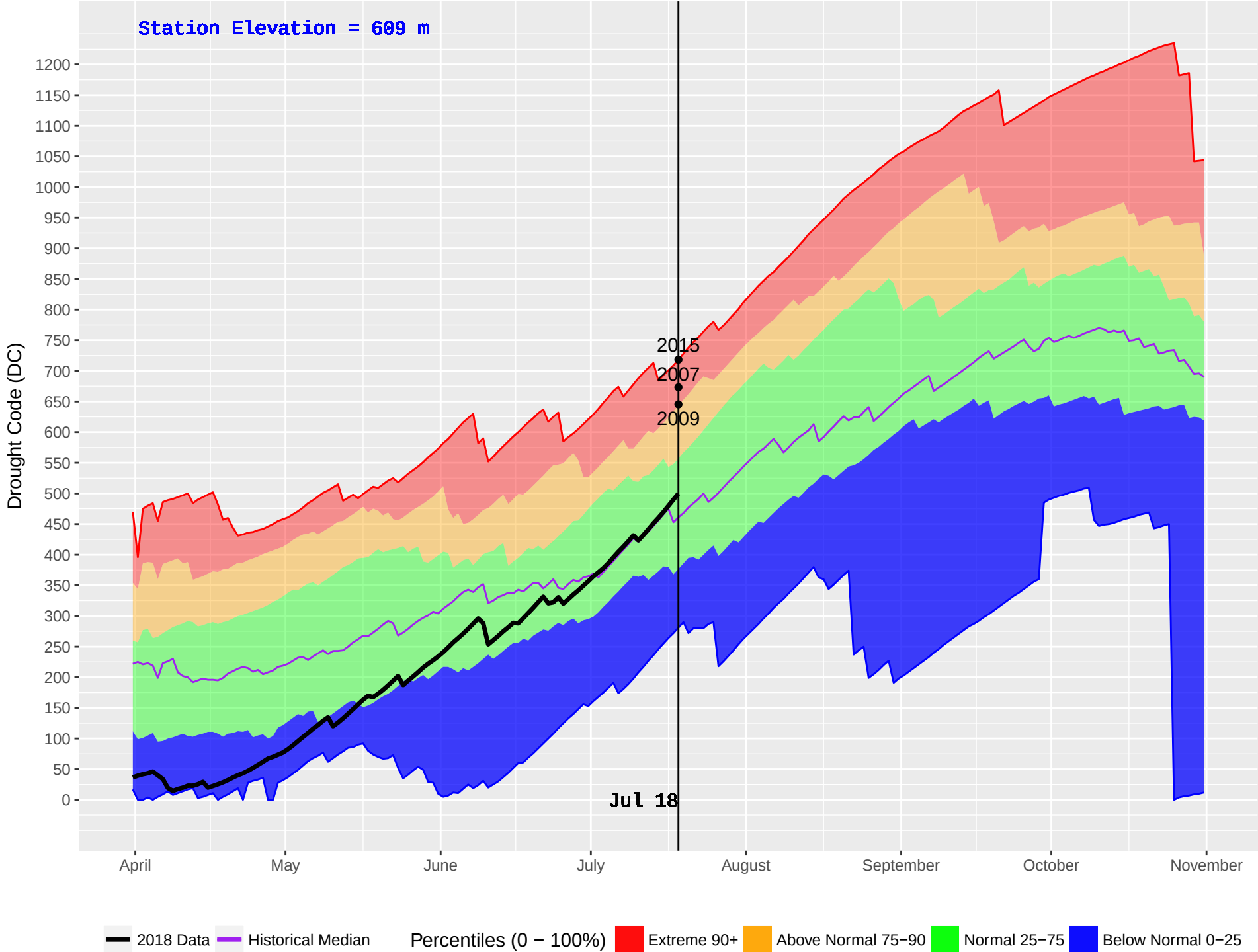
ROCK CREEK (394) : Historical (1990–2016) and Current (2018) Daily Drought Code (DC)
