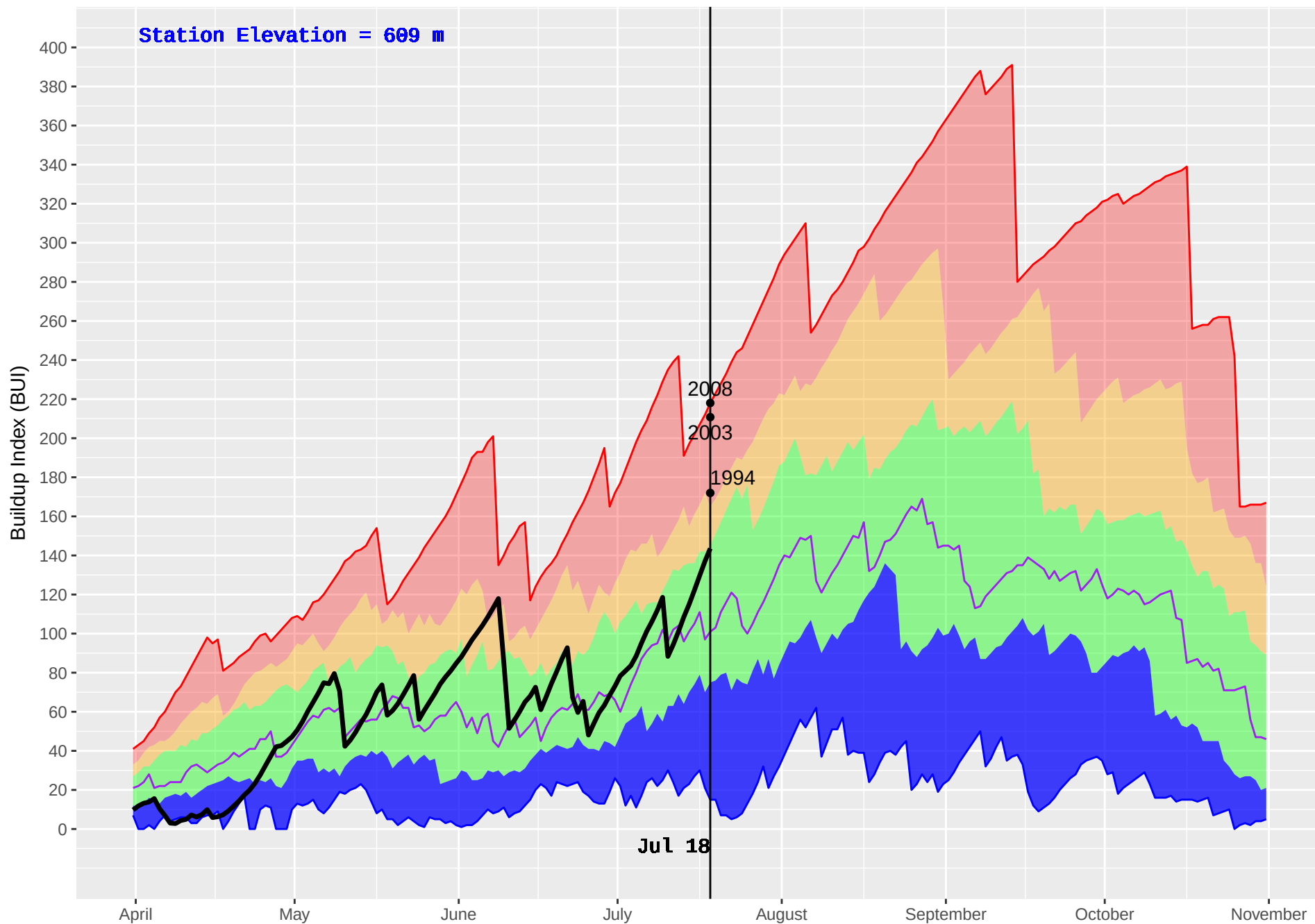
ROCK CREEK (394) : Historical (1990–2016) and Current (2018) Daily Buildup Index (BUI)
