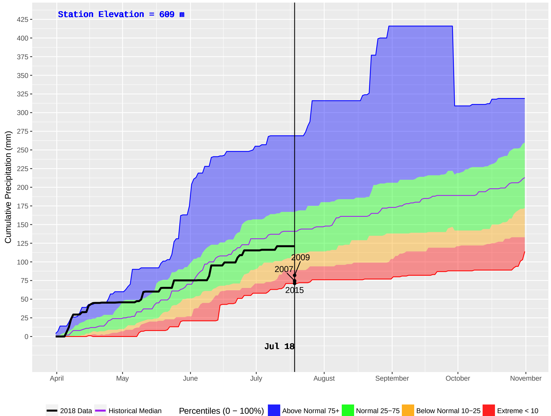
ROCK CREEK (394) : Historical (1990–2016) and Current (2018) Daily Cumulative Precipitation
